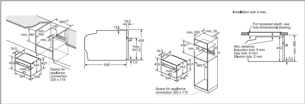
Steam ovens CBG675BS1B | CSG656BS6B | CDG634BS1B | CNG6764S6B | CMG656BS6B | CMG633BS1B | CMG676BS6B | CMG656BB6B | CMG633BB1B
