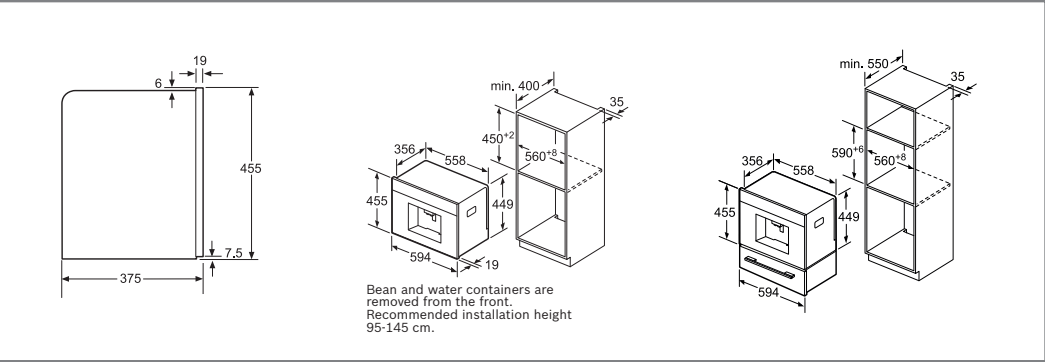
Coffee maker CTL636ES6
