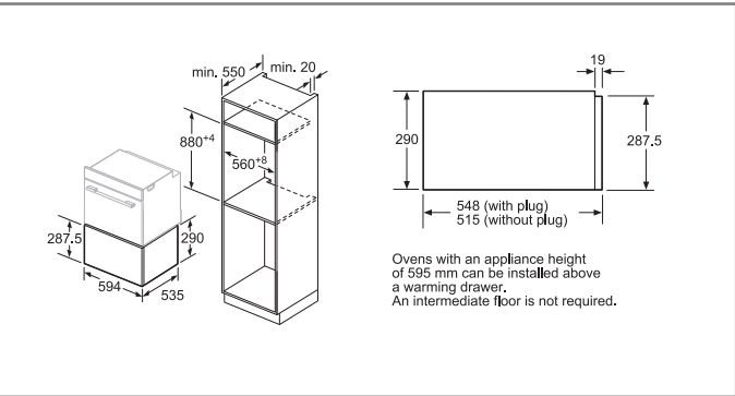
Warming drawer BID630NS1B installed with 60cm high single oven.
