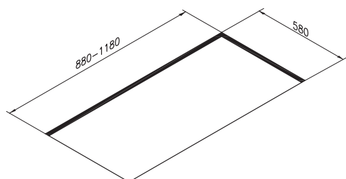
With F13 Motor
